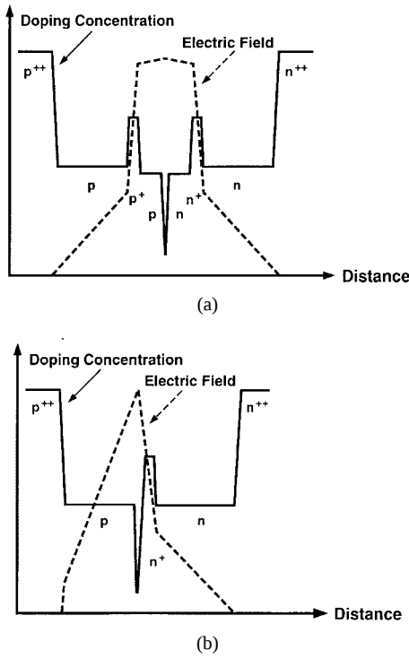
Fig. 8. Schematic doping profiles for high-power high-efficiency double-drift IMPATT diodes. (a) Double-drift Hybrid Read low-high-low. (b) Double-drift Hybrid Read flat-high-low.
