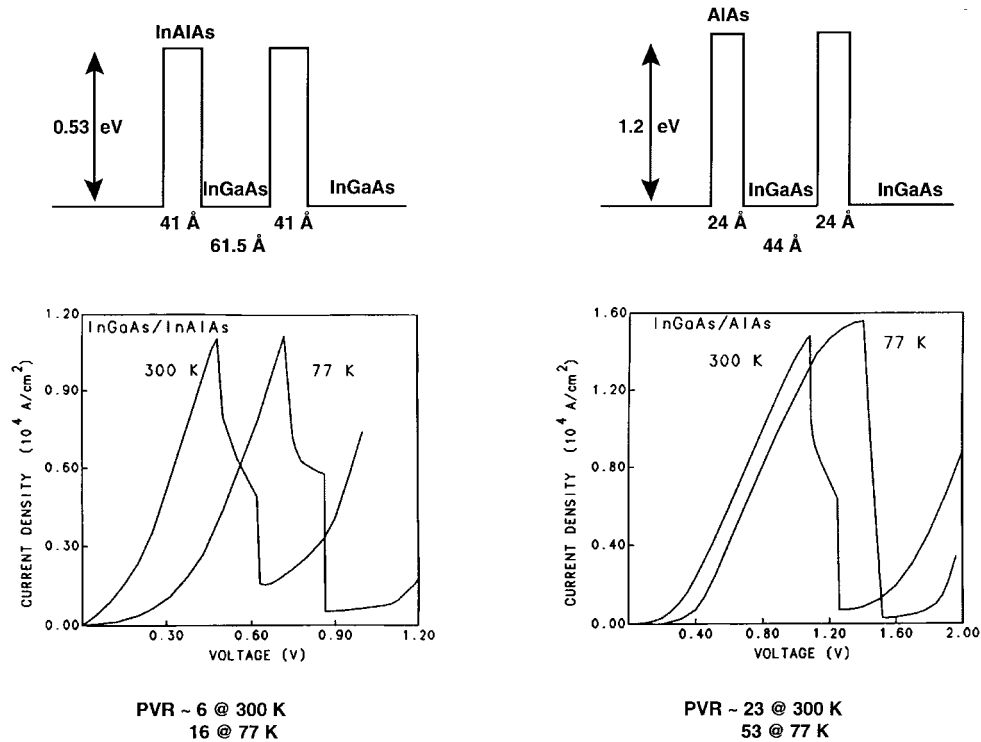
Fig. 2. Conduction band profiles and current-voltage characteristics for lattice-matched InAlAs/InGaAs and strained AlAs/InGaAs RTD's with high PVR's.
